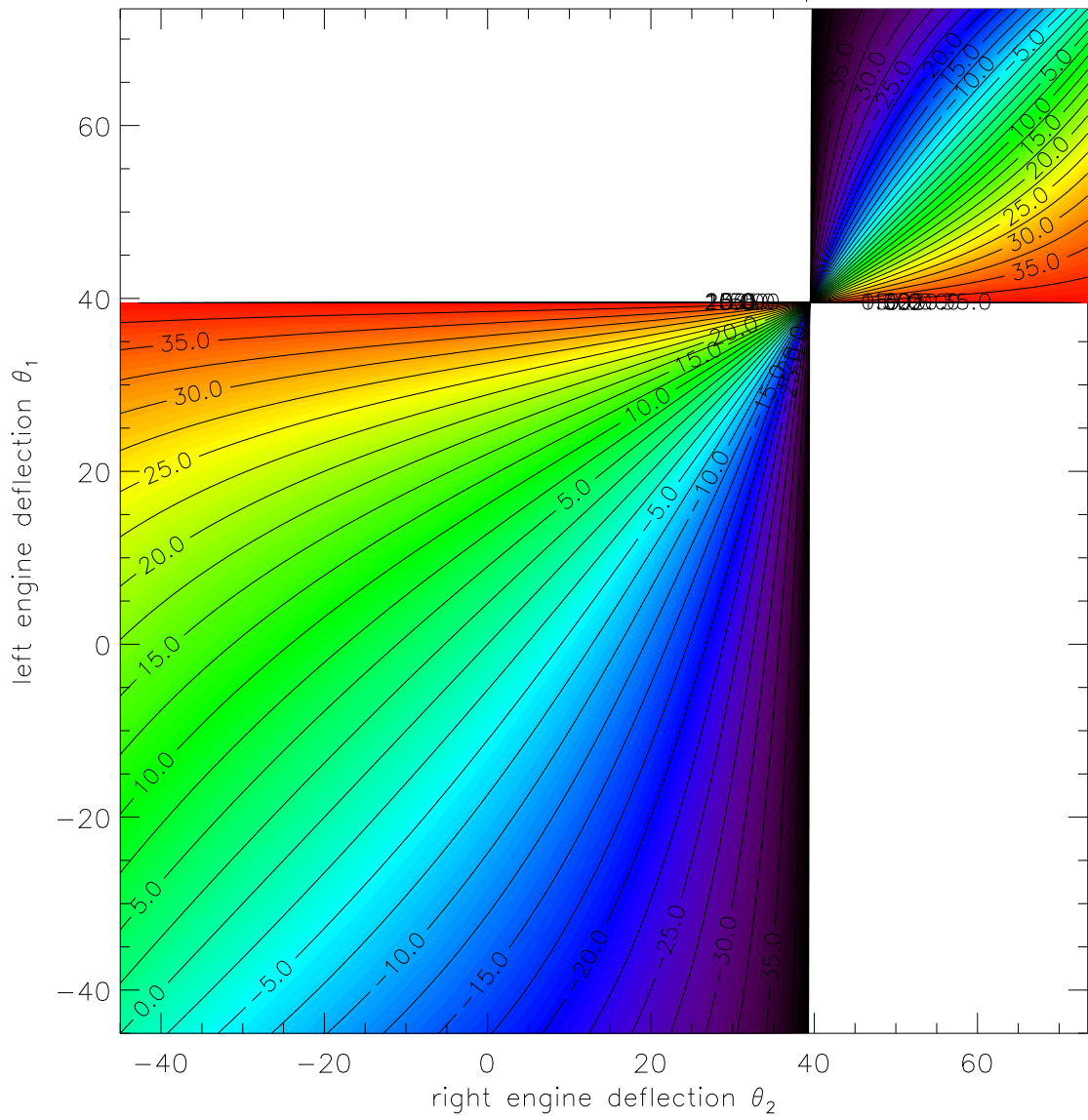
thrust direction: TIE Interceptor
