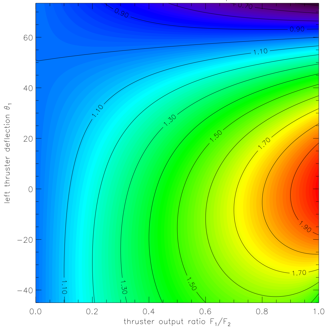
total thrust: TIE Interceptor
