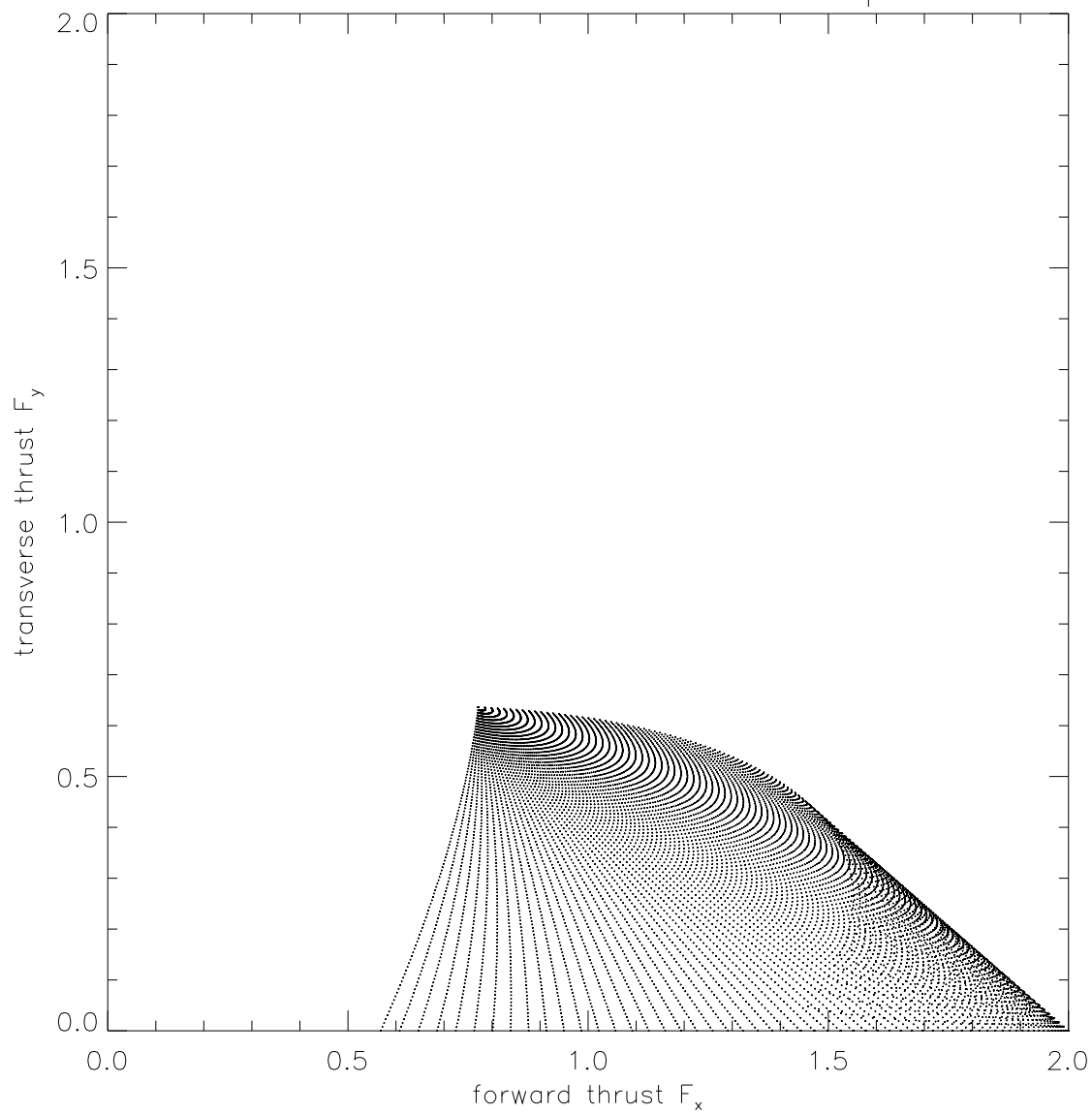
attainable thrust vectors: TIE Interceptor
